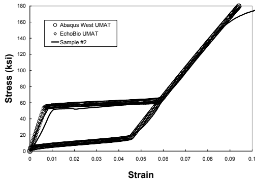
Figure 2. Comparison of FEA predictions and the experimental data
