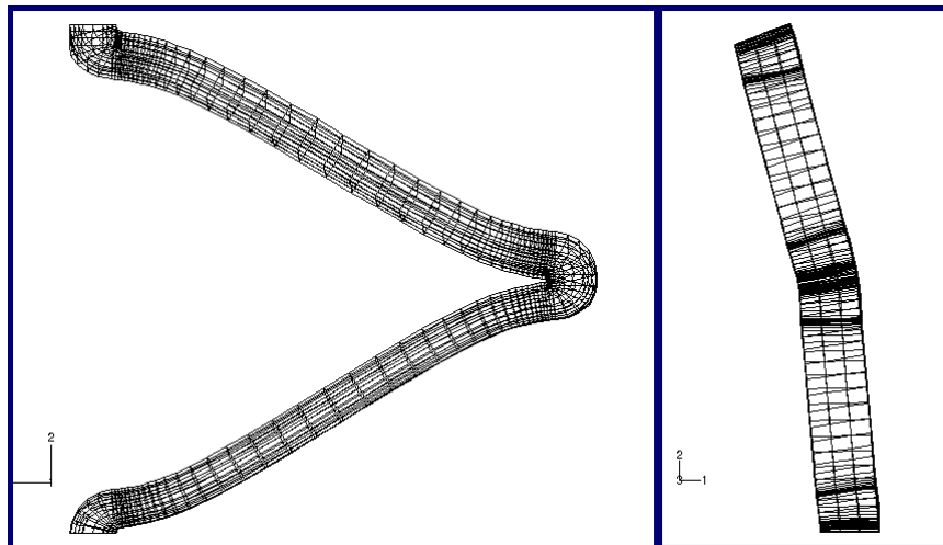
Figure 4. Side (left) and top (right) views of a two strut model
