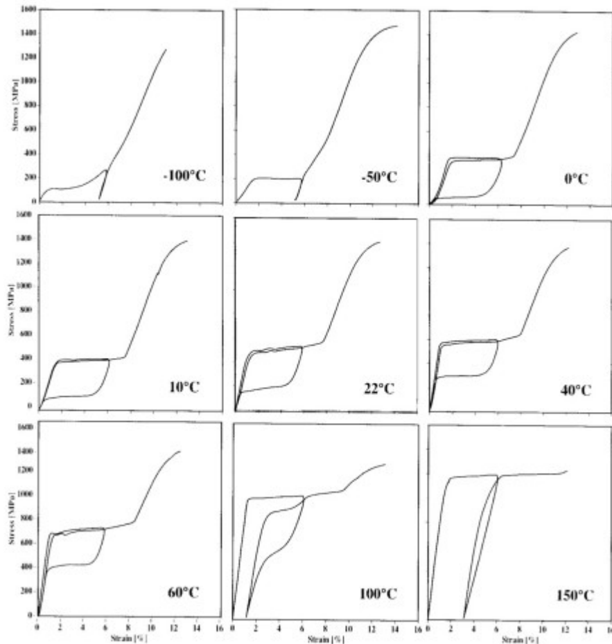
Figure 1. Uniaxial stress-strain relation at different temperatures
