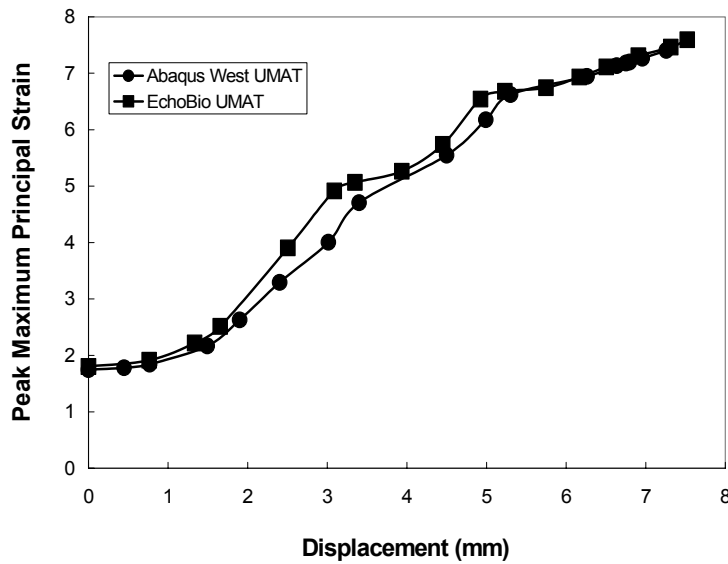
Figure 11. Peak maximum principal strain as function of displacement from two different material models
