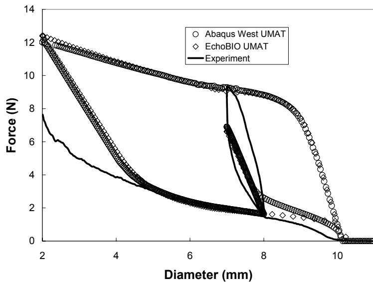
Figure 5. Comparisons of FEA predictions and the tests results
