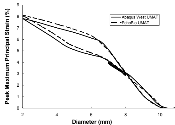
Figure 7. Peak maximum principal strain as function of stent diameter
