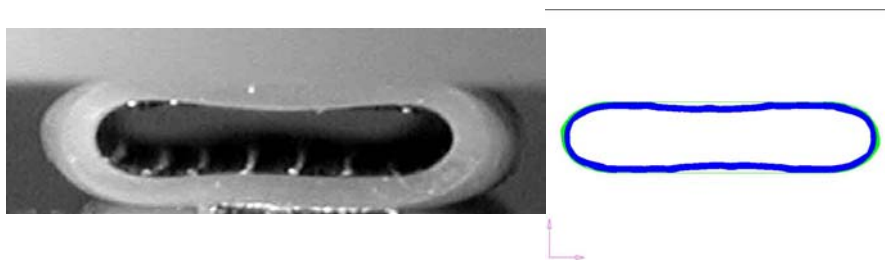
Figure 9. Comparison of deformed stent shape from experiment (left) and FEA (right)
