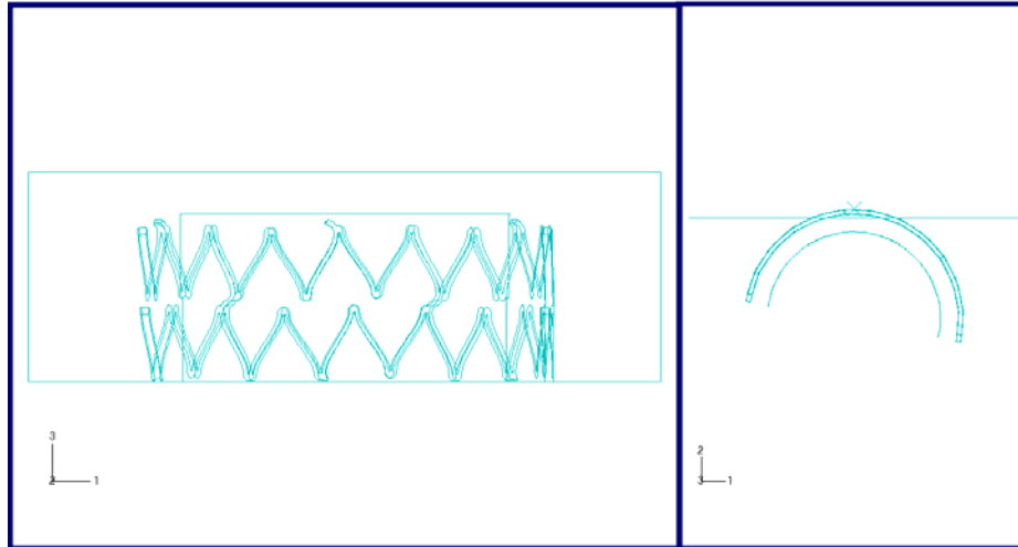
Figure 8. Side (left) and top (right) views of the FEA model for crush simulation
