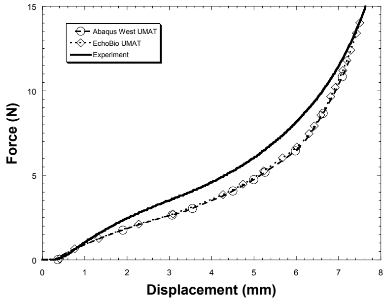
Figure 10. Comparison of force-displacement relations from experiment and FEA
