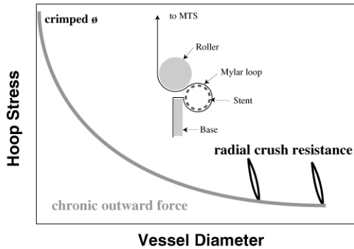
Figure 3. Schematic radial stiffness test set up
